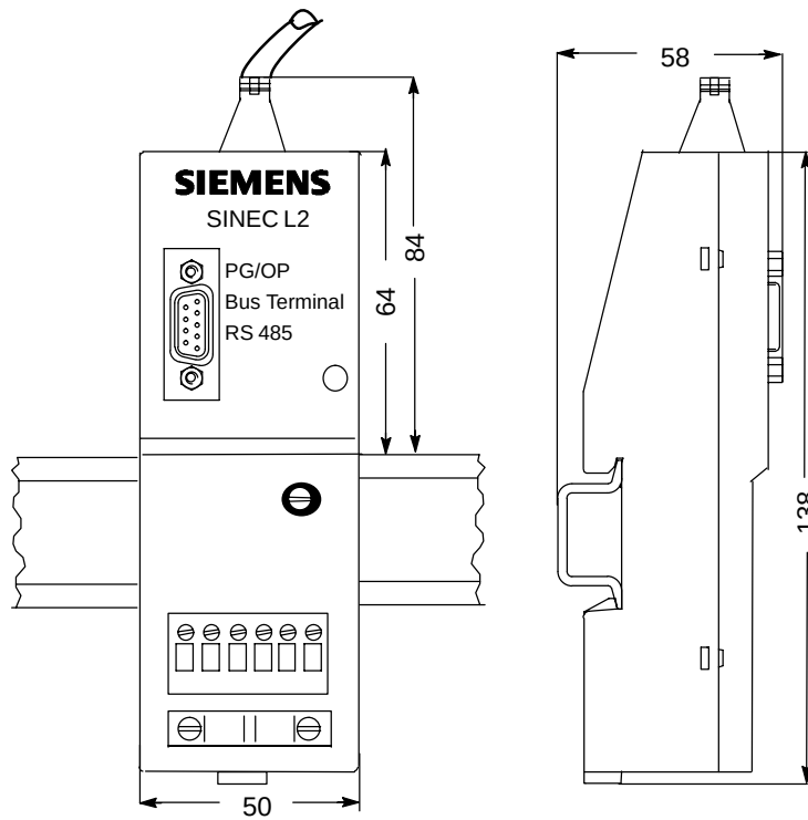
Figure E-10 RS-485 Bus Terminal on 15 mm high Standard Rail
