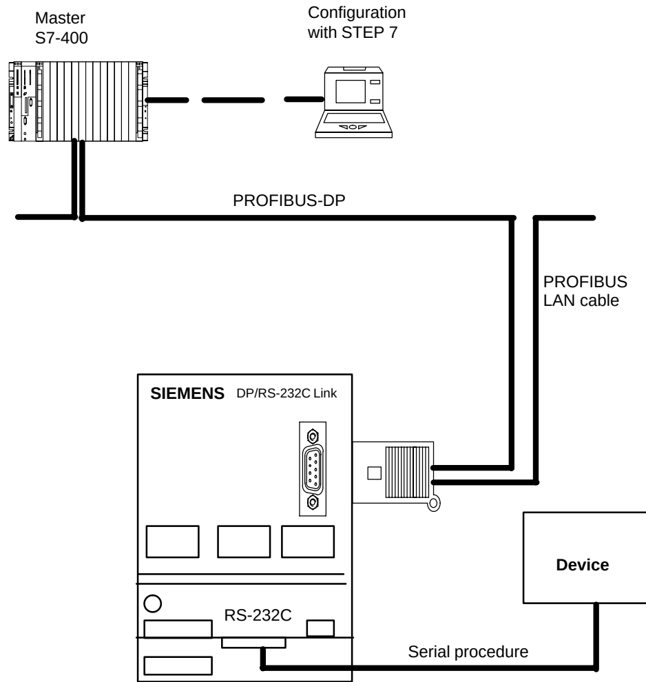
Figure 2-20 Example of a Configuration with DP/RS-232C Link
