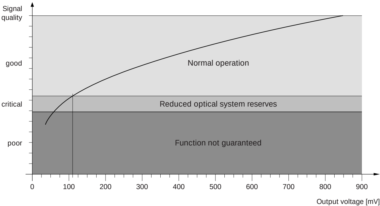
Diagram 1: Assignment of measured output voltage to signal quality for the OLM/G11, OLM G/12 and OLM/G12-EEC
