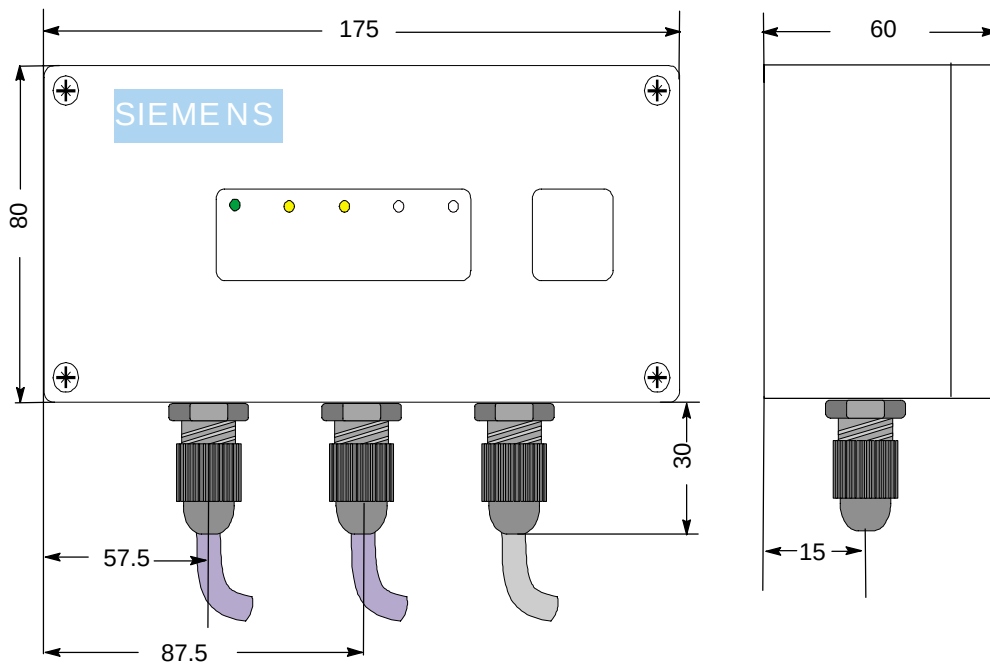
Figure E-14 PROFIBUS ILM
