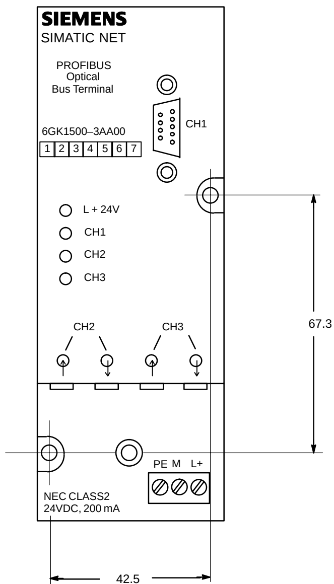
Figure E-13 Drilling Template for the Optical Bus Terminal OBT
