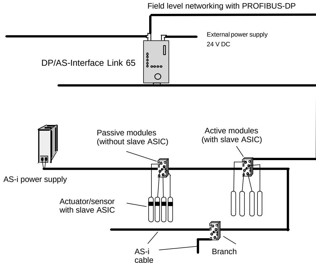
Figure 2-22 Example of a Configuration with DP/AS-Interface Link 65
