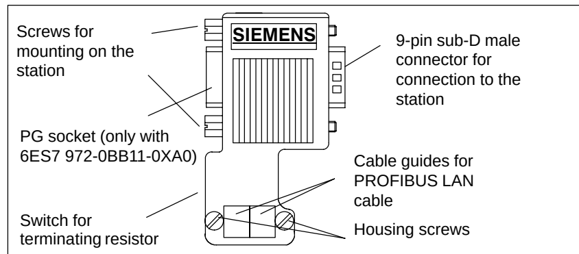
Figure 4-15 Bus Connector (order number 6ES7 972-0B.11 ...)
