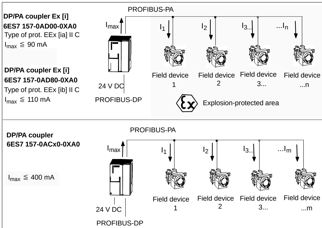
Figure 2-13 Field Device Power Supply in the Hazardous and Non-Hazardous Area
