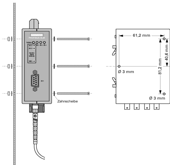
Figure E-18 Mounting the Optical Link Module OLM on a Mounting Plate
