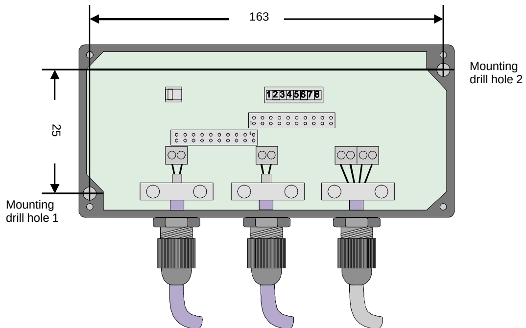
Figure E-15 Drilling Dimensions for Securing the PROFIBUS ILM to a Mounting Plate
