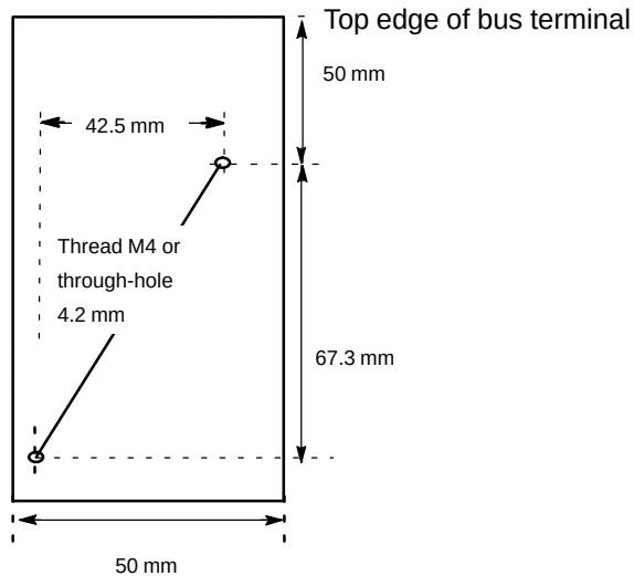
Figure 4-31 Drilling Diagram for the Bus Terminal
