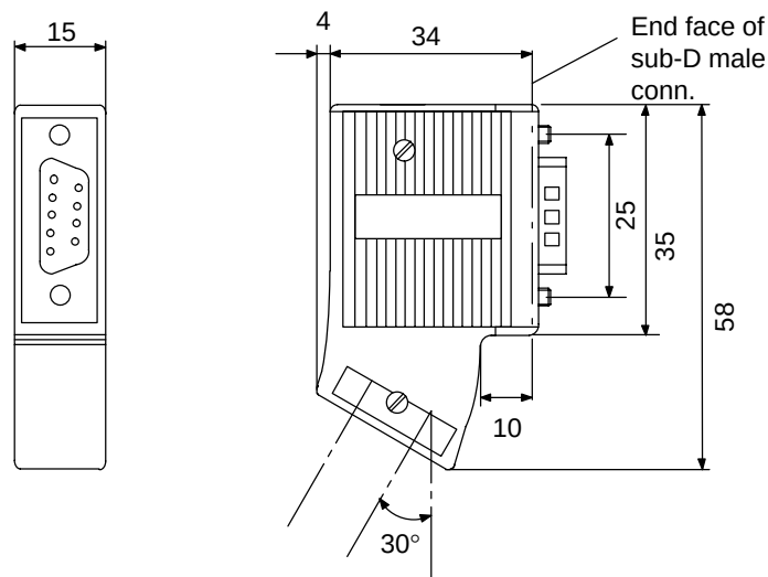
Figure E-2 Bus Connector to IP 20 (6ES7 972-0BA30-0XA0)
