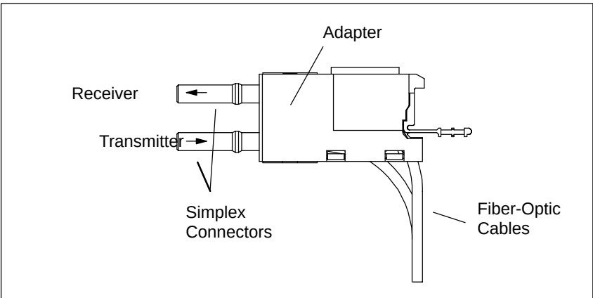
Bild 7-9 Simplex Connector and Special Adapter Fitted Together
