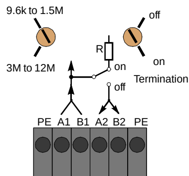
Figure 4-30 Operator Controls
