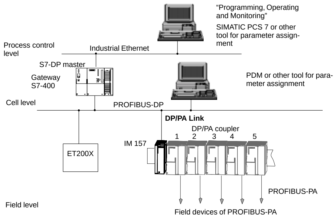
Figure 2-17 Location of the DP/PA Link
