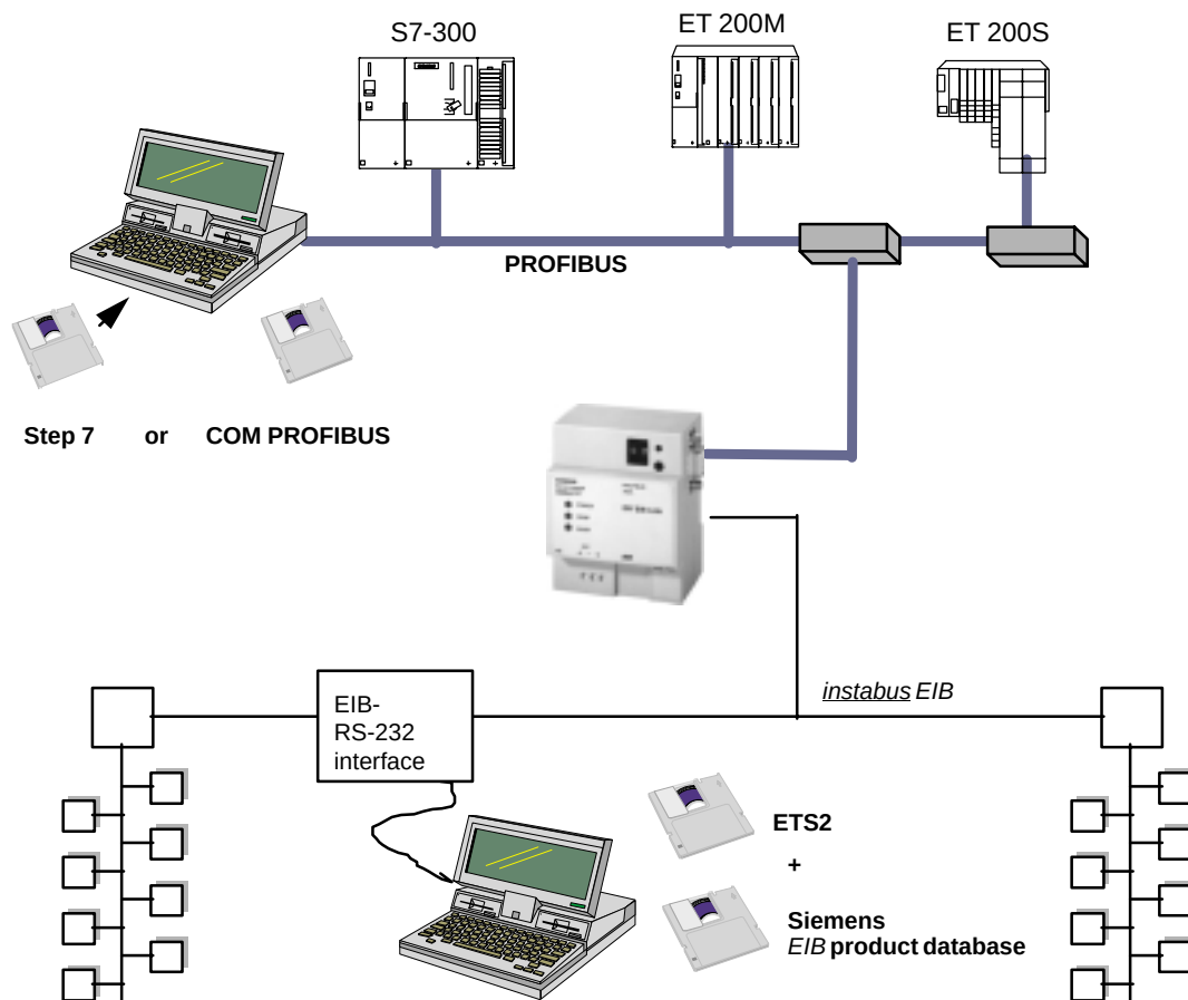
Figure 2-26 Example of a System Structure using DP/EIB Link
