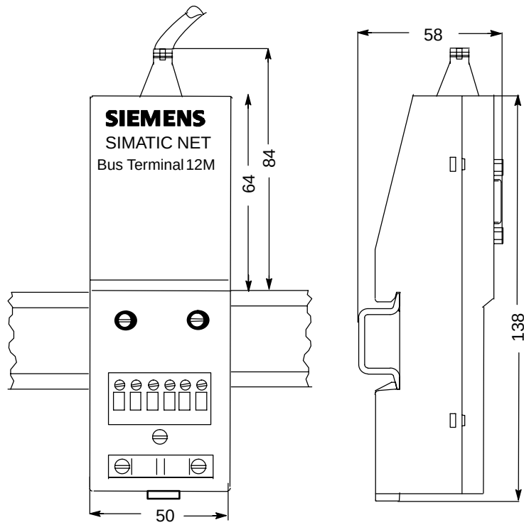
Figure E-11 BT12M Bus Terminal on 15 mm high Standard Rail
