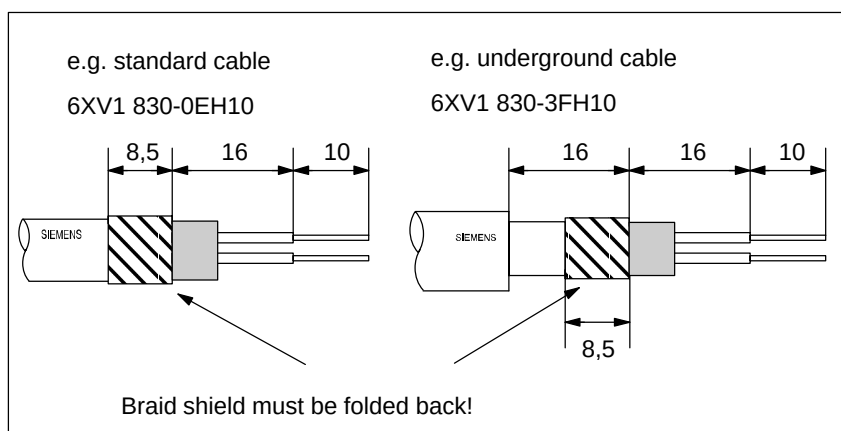
Figure 5-10 Stripping the Insulation to Connect to the PROFIBUS Terminator
