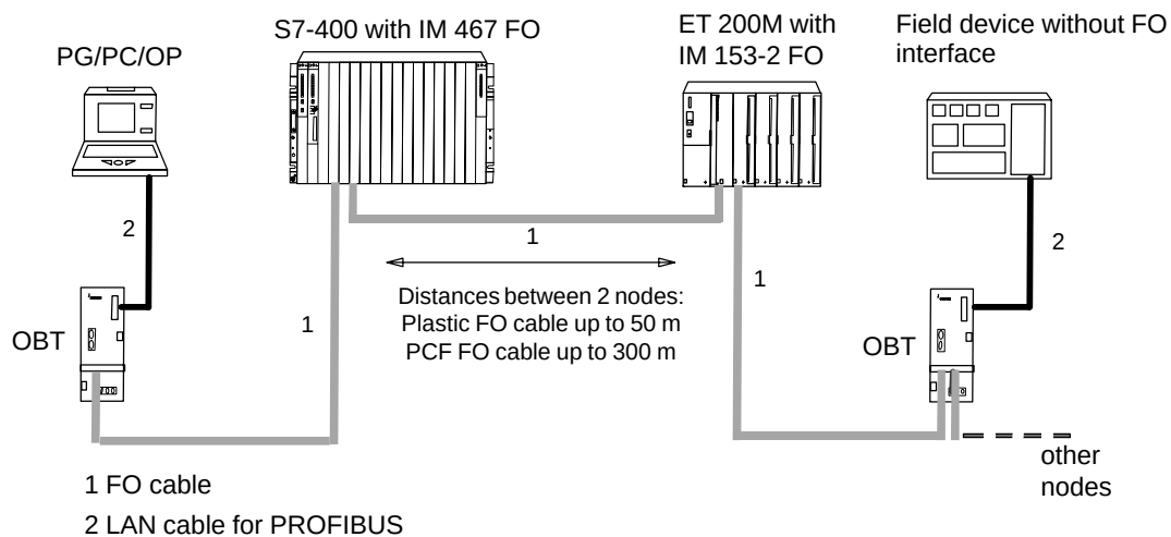
Figure 2-2 PROFIBUS DP Network with Nodes Having Integrated FO Interfaces
