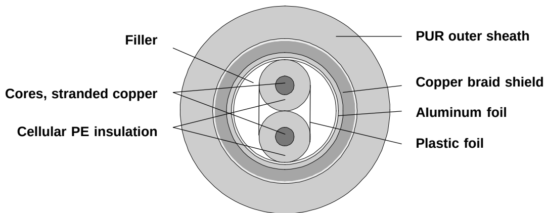
Figure 4-7 Structure of the Trailing Cable
