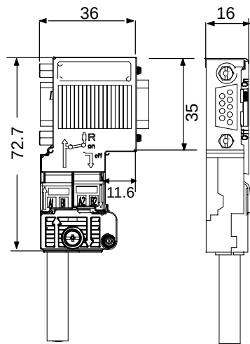
Figure E-5 FastConnect Bus Connector (6ES7 972-0B.50-0XA0)
