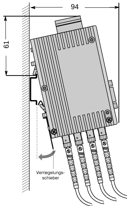
Figure E-17 Mounting the Optical Link Module OLM on a 7.5 mm high Standard Rail
