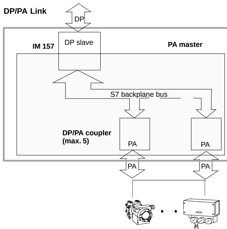
Figure 2-18 The DP/PA Link with DP/PA Couplers
