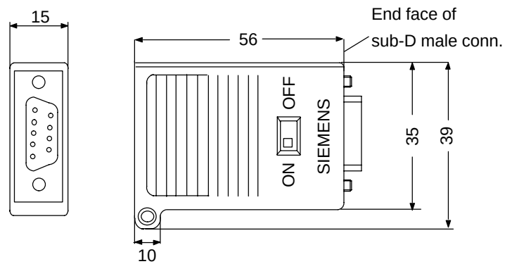
Figure E-4 Bus Connector to IP 20 (6GK1 500-0EA02)
