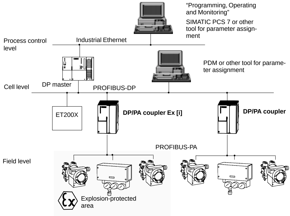
Figure 2-16 Linking the DP/PA Coupler into the System
