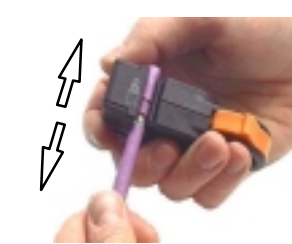
6. Keeping the tool closed, remove it from the end of the cable. If the cut is poor, change the blade cassette.
