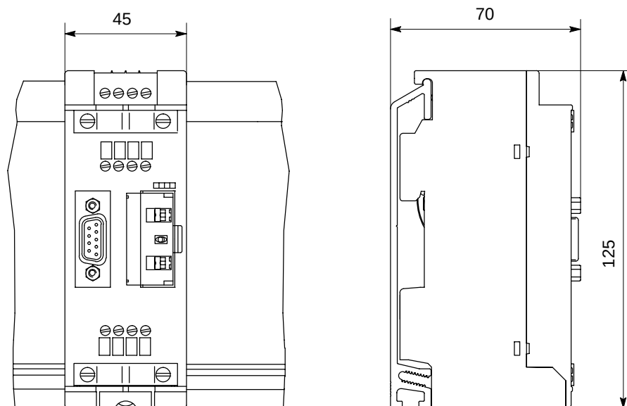
Figure E-8 RS-485 Repeater on S7-300 Rail
