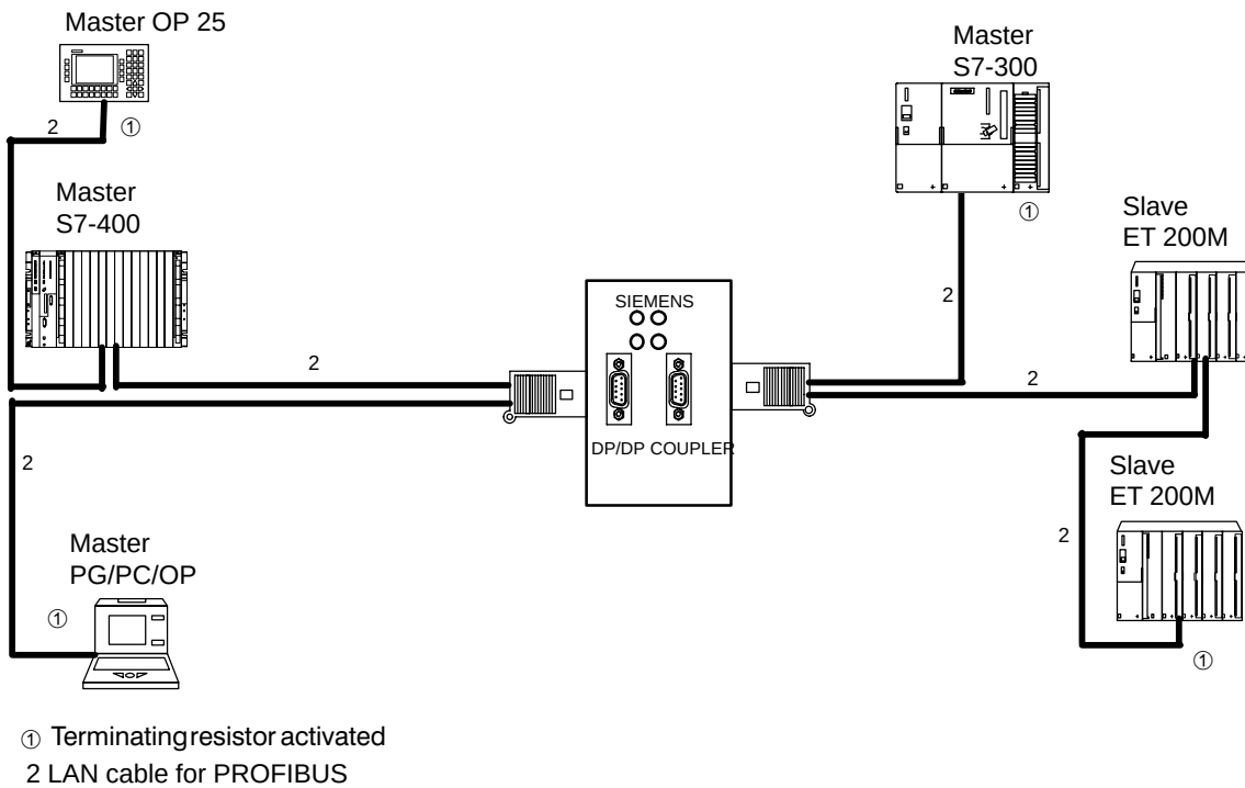
Figure 2-15 Configuration Example of the DP/DP Coupler
