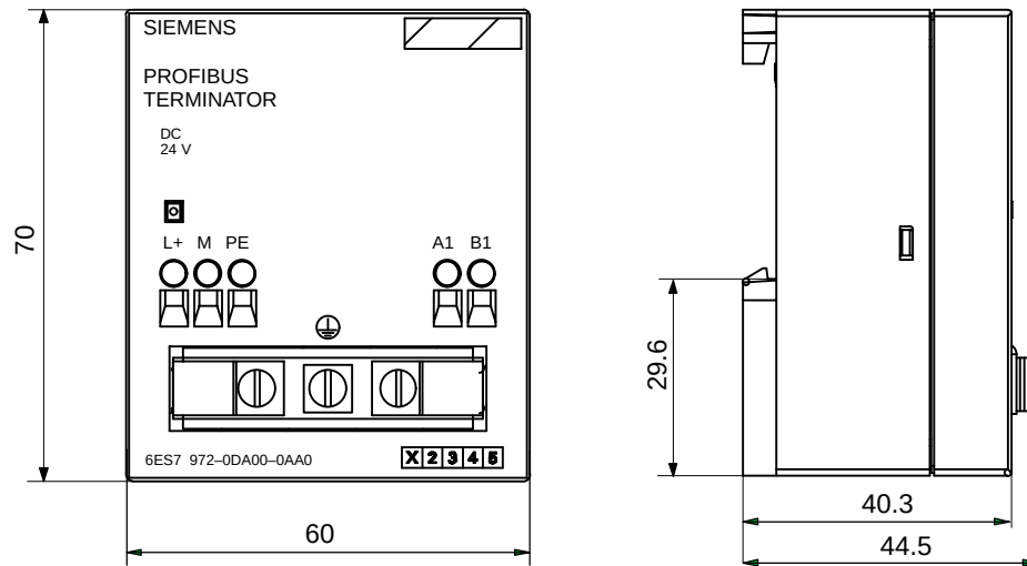
Figure E-9 PROFIBUS Terminator
