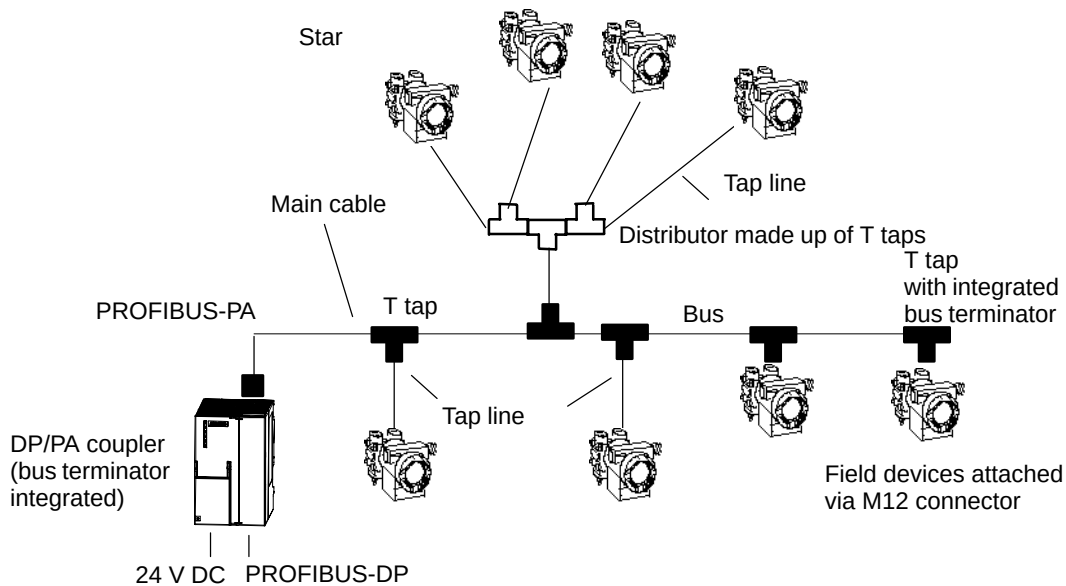
Figure 2-12 Bus and Star Topology
