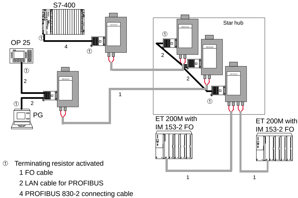
Figure 2-4 Example of a Star Topology with OLMs
