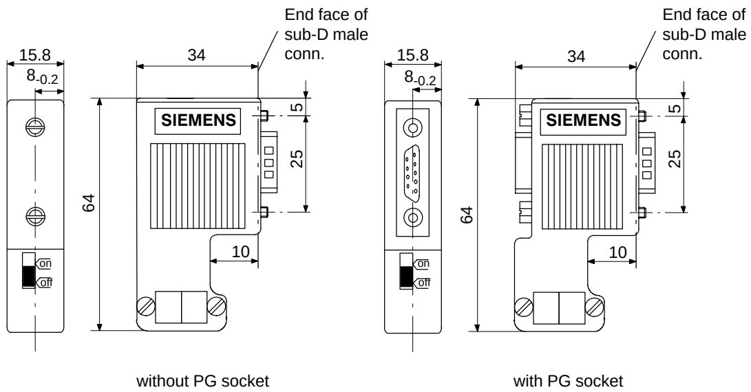
Figure E-1 Bus Connector to IP 20 (6ES7 972-0B.11-0XA0)
