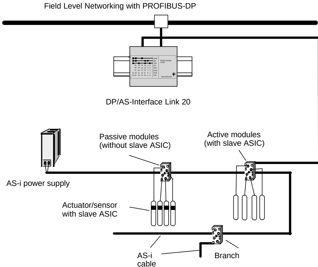
Figure 2-24 Example of a Configuration with DP/AS-Interface Link 20
