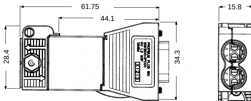
Figure E-6 FastConnect Bus Connector (6GK1 500-0FC00)
