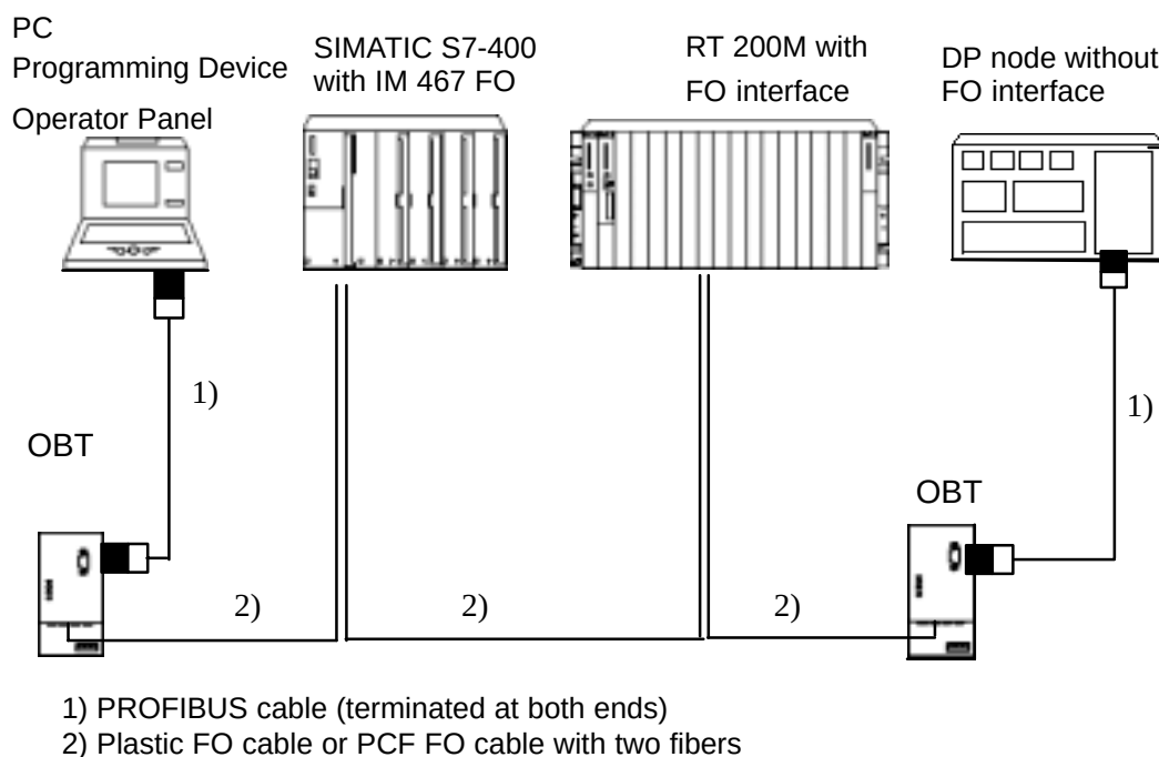
Figure 1-1 Example of an Optical PROFIBUS DP Configuration
