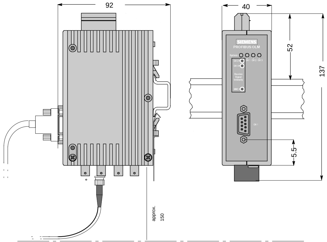
Figure E-16 Optical Link Module OLM on 15 mm high Standard Rail
