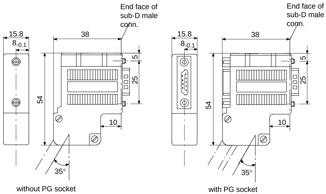
Figure E-3 Bus Connector to IP 20 (6ES7 972-0B.40-0XA0)
