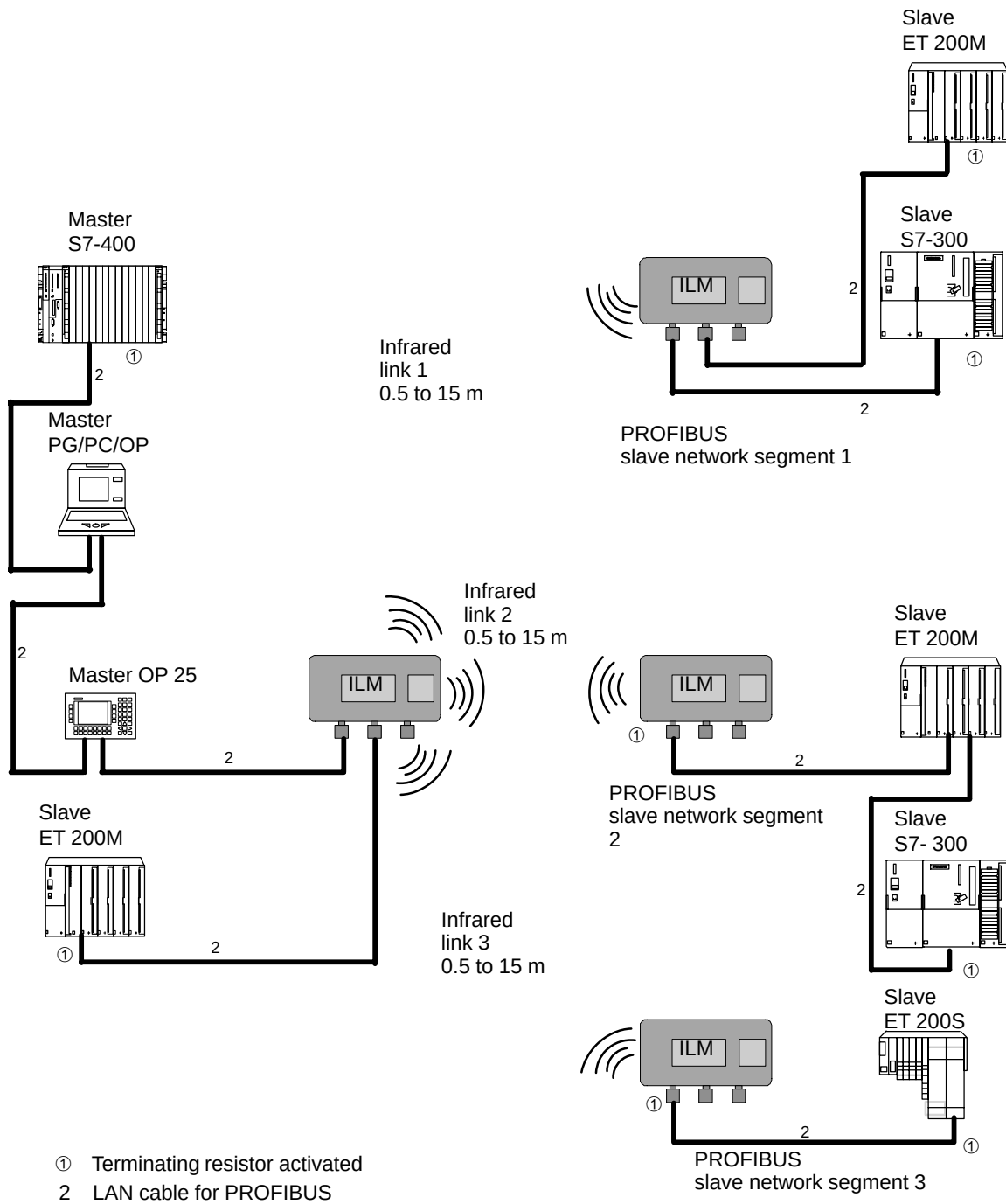
Figure 2-11 Point-to-Multipoint Link Using PROFIBUS ILMs (One Master Subnet, Three Subnets with Slaves)
