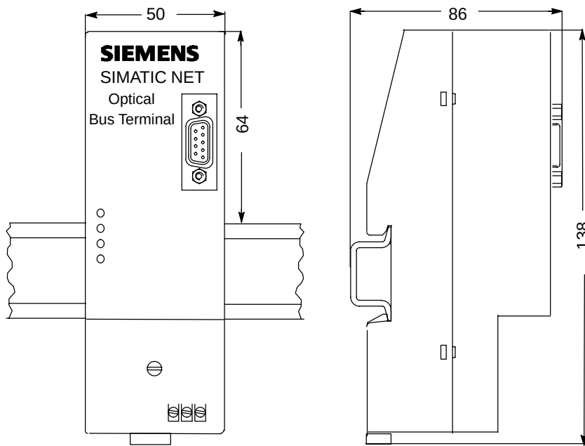
Figure E-12 Optical Bus Terminal OBT on 15 mm high Standard Rail
