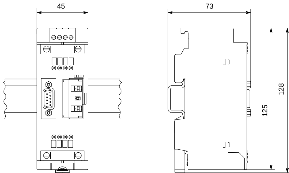
Figure E-7 RS-485 Repeater on Standard Rail
